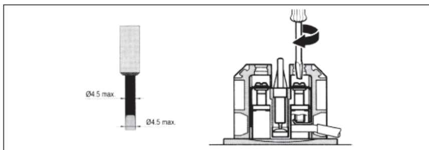
Figure 6: Fixing the supply cable.
